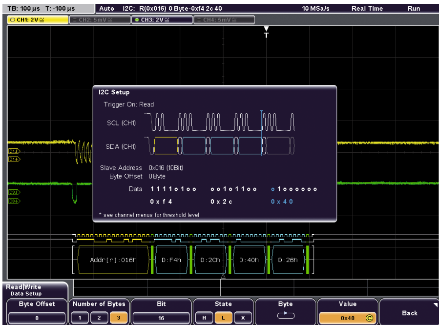
Decoded hexadecimal I 2 C message.
