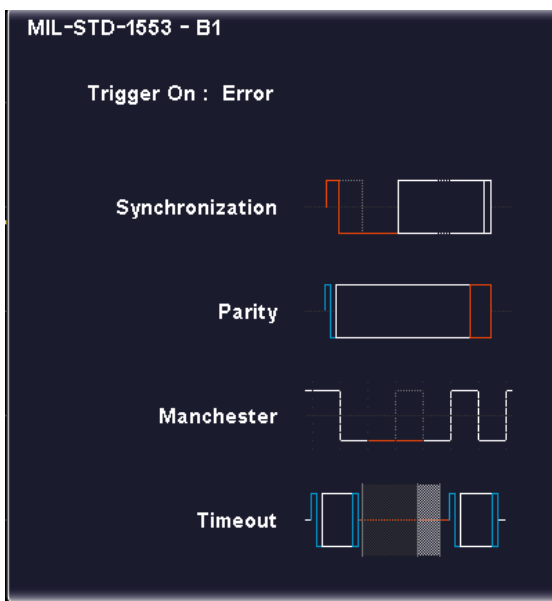
Communicative popup windows: intuitive display of setting options for error states in the MIL-STD-1553 protocol.
